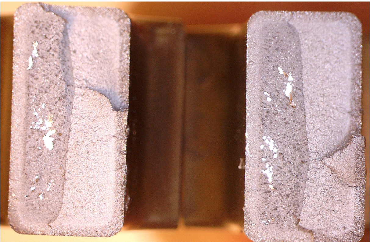
Figure 6: Fracture surface of specimen IT201-15, 2N_f=5,936
