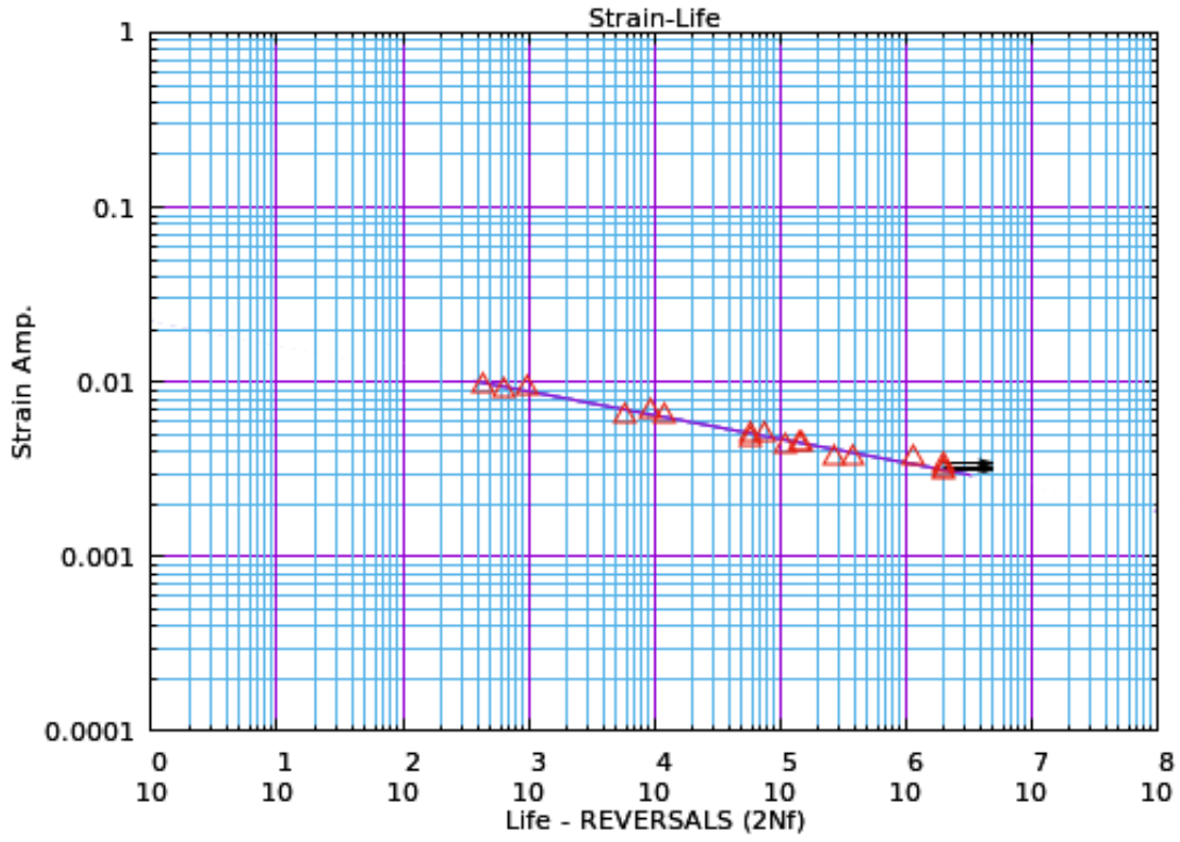
Figure 4: Strain-life fatigue curve for AISI 16MnCr5 modified case/core composite 1900F (IT 201)
