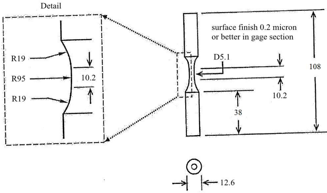
Figure 5: Specimen configuration and dimensions (mm)
