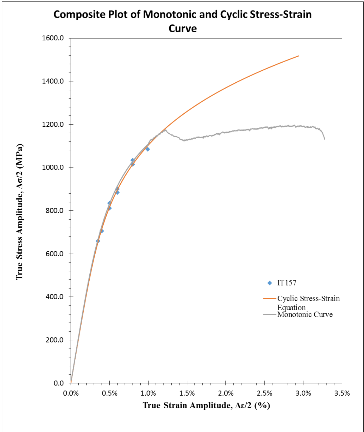
Figure 10: Composite plot of cyclic and monotonic stress-strain curves
