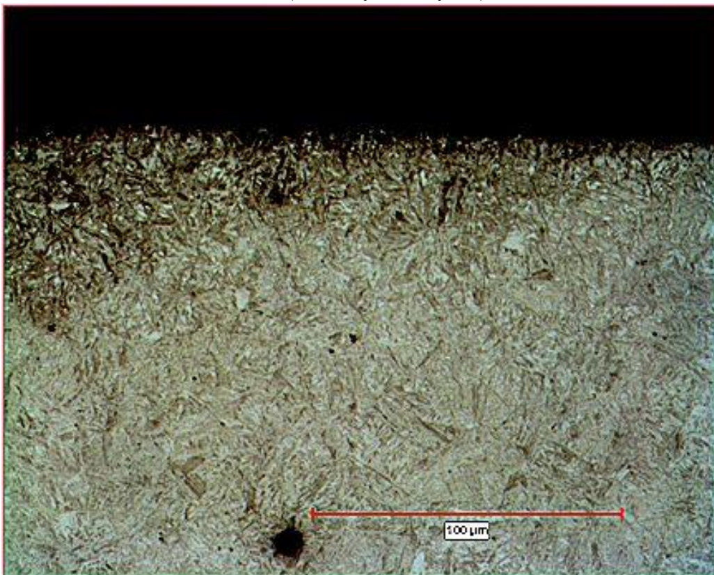
Figure 2: High magnification photograph of the inclusion distribution in the case area (Courtesy of Chrysler)
