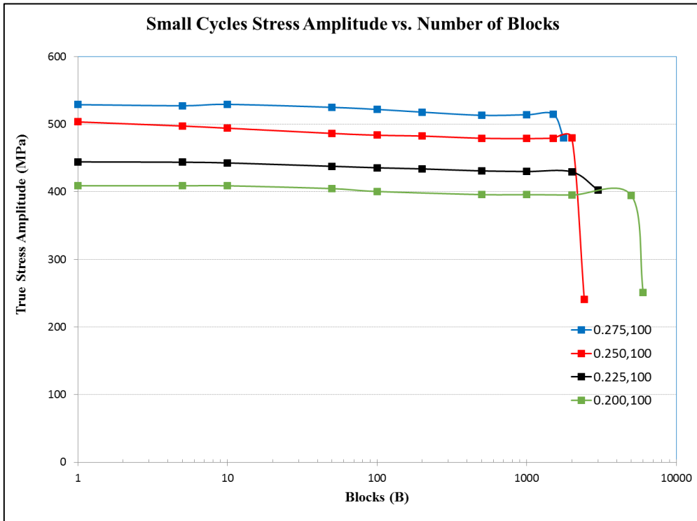
Figure A.3a: Small cycle amplitude transient response throughout the life
