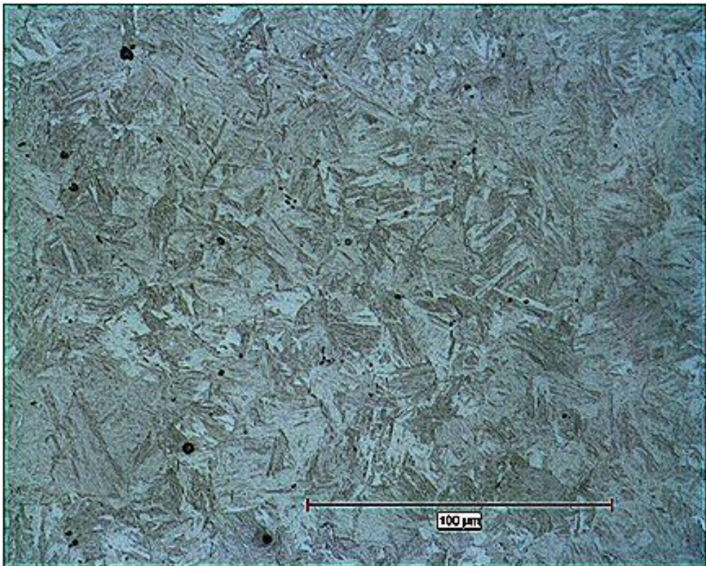
Figure 4: High magnification photograph of the inclusion distribution in the core area (Courtesy of Chrysler)
