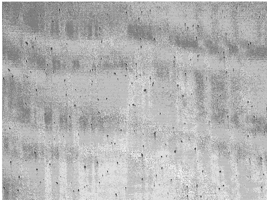
Figure 3b: Examples of inclusions in the transverse direction (T-T) at 100X for SAE 4140 (0.077S) steel (rolling direction is perpendicular to the page).
