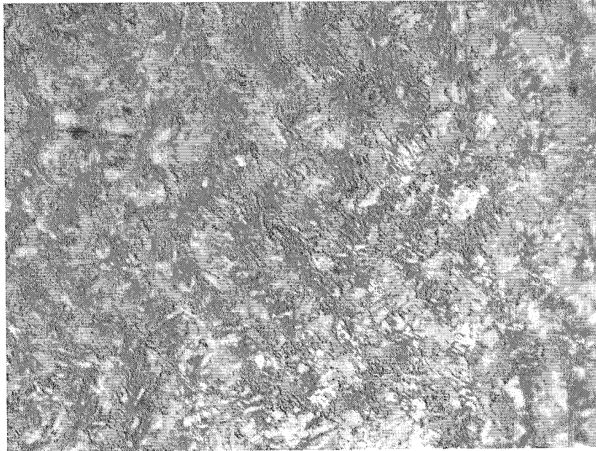
Figure 2a: Photomicrograph in longitudinal direction (L-T) at 500X for SAE 4140 (0.077S) steel (rolling direction is parallel to the page).
