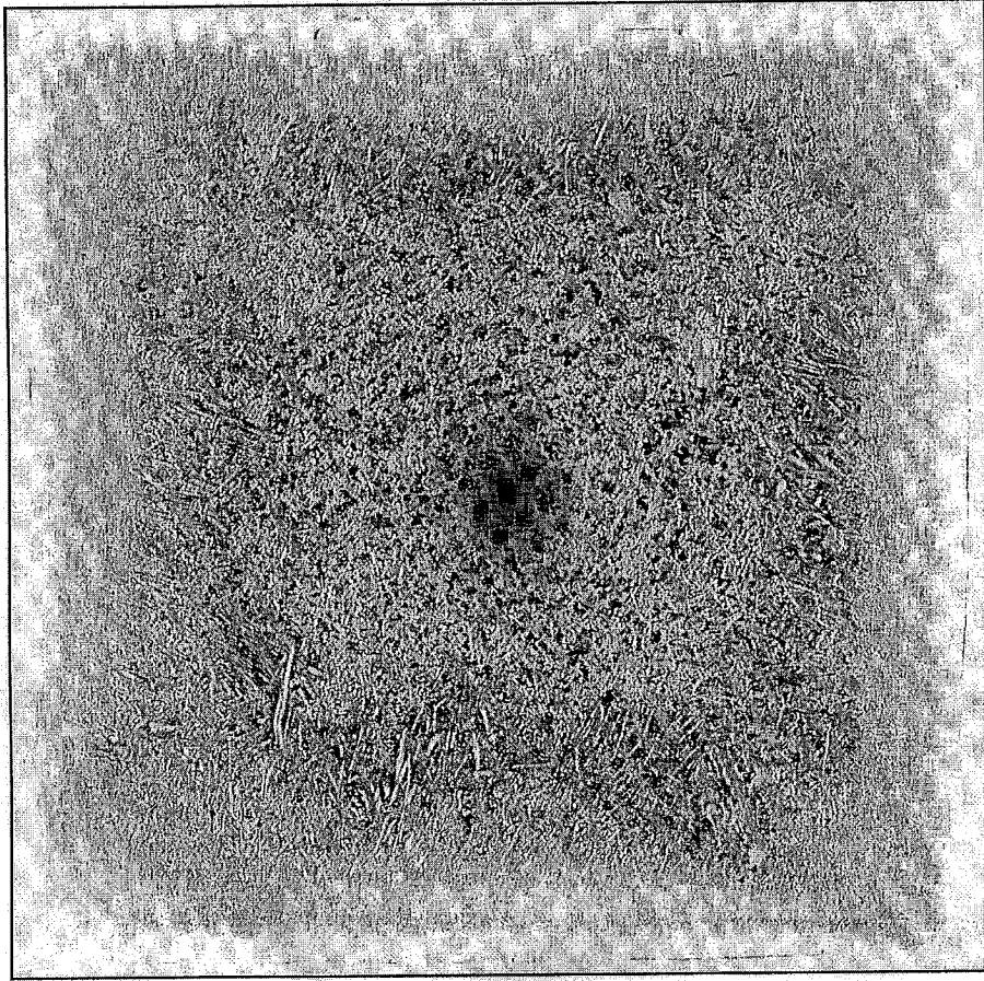
Figure 1d: Sulfur printing of SAE 4140 High sulfur (0.077% max S) steel (Provided by Macsteel – Monroe Division)
