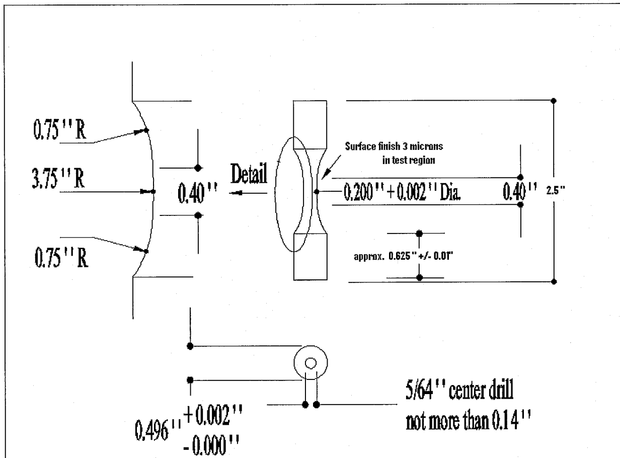
Figure 1a: Specimen configuration and dimensions
