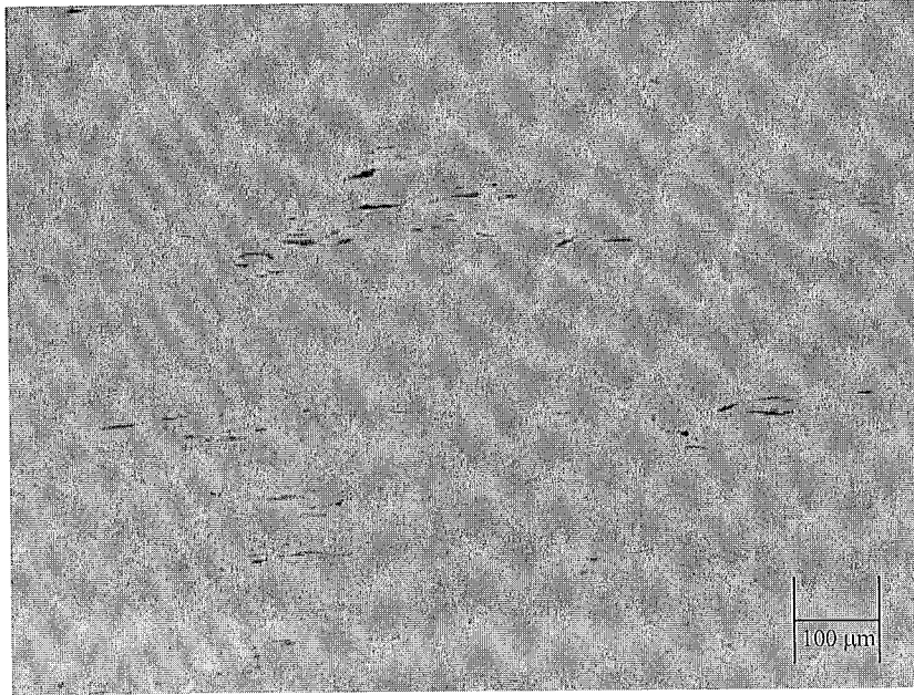
Figure 3: Sulfide inclusions in 2.5" square bars Heat M14218 – 0.077% S (original 100X) Rated as A thin = 3.5 and A heavy = 1.0, D thin = 1.0 and D heavy = 0.5 (no B or C) (Provided by Macsteel Company – Monroe Division)
