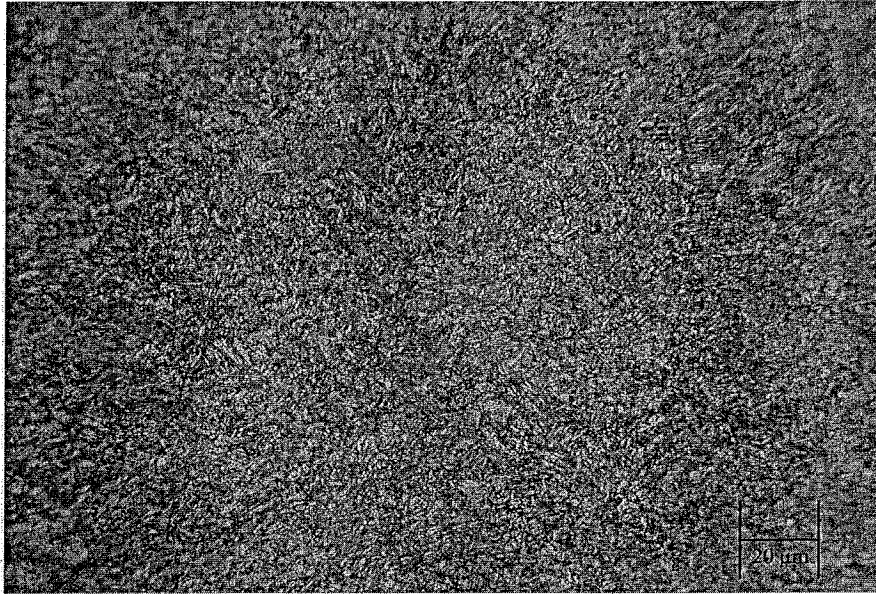
Figure 2: Photomicrograph in the direction perpendicular to applied axial load (L-T as shown in Fig. 1(c)) at 500X for SAE 4140 Low S (0.012% max.) steel.
