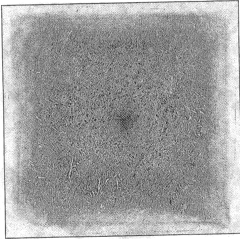
Figure 1d: Sulfur printing of heat no.14218 (It 77)(Provided by Macsteel – Monroe Division)
