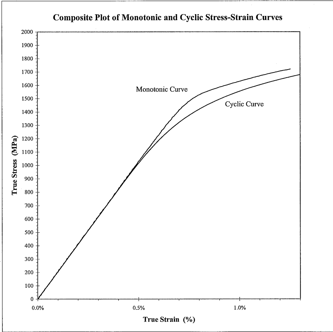
Figure 8: Composite plot of cyclic and monotonic stress-strain curves
