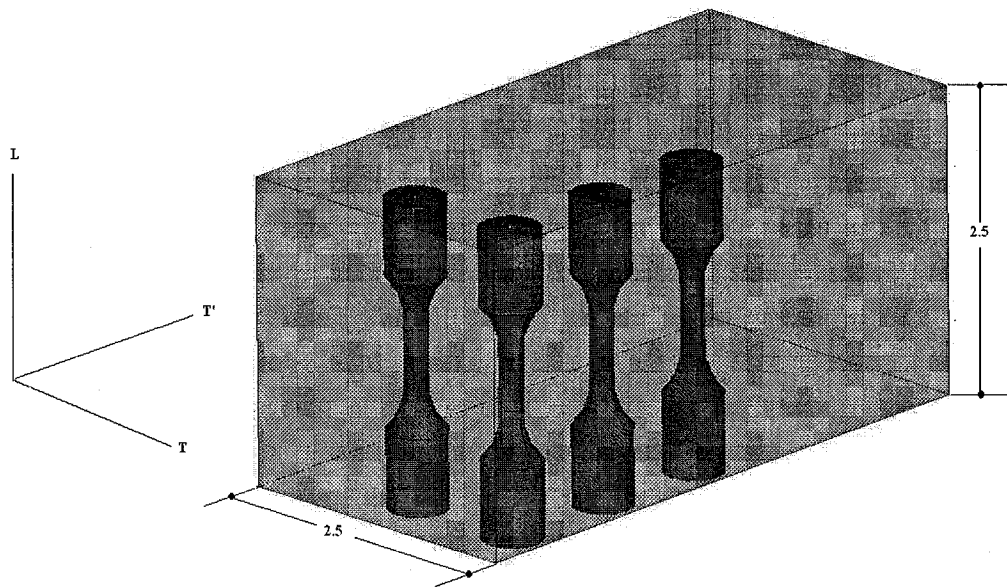
Figure 1c: Sample cut-out direction
