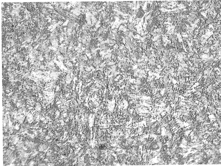
Figure 2a: Photomicrograph in longitudinal direction (L-T) at 500X for SAE 86B20 Quenched Core (Atm) steel (rolling direction is parallel to the page).
