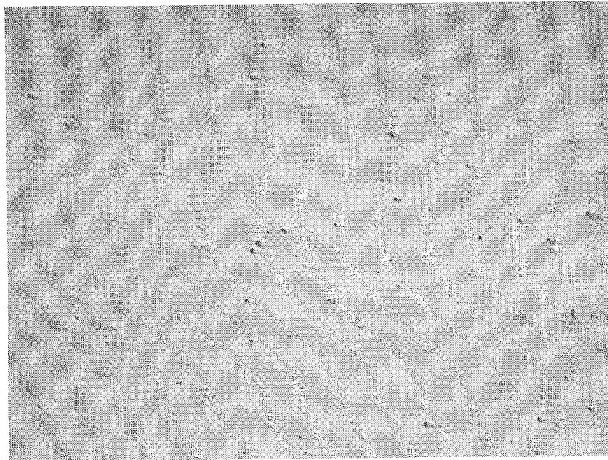
Figure 3a: Examples of inclusions in the longitudinal direction (L-T) at 100X for SAE 86B20 Quenched Core (Atm) steel (rolling direction is parallel to the page).
