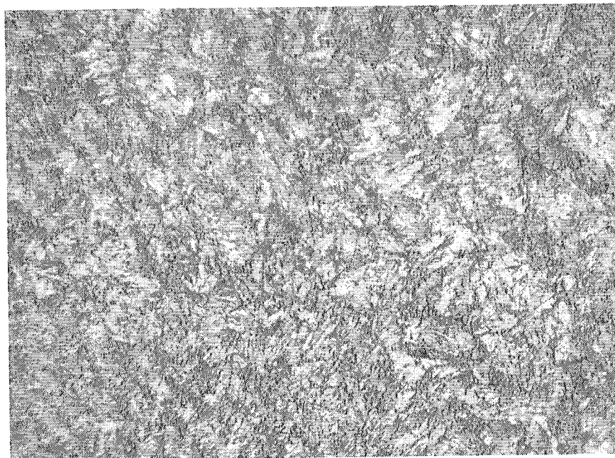
Figure 2b: Photomicrograph in transverse direction (T'-T) at 500X for 86B20 Quenched Core (Atm) steel (rolling direction is perpendicular to the page).
