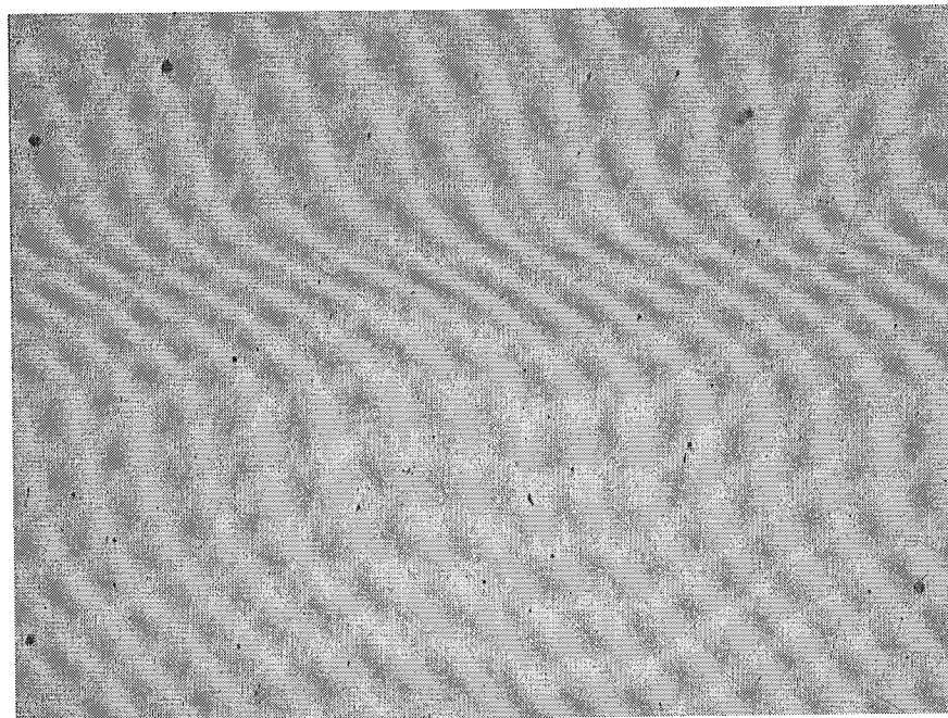
Figure 3b: Examples of inclusions in the transverse direction (T'-T) at 100X for SAE 86B20 Quenched Core (Atm) steel (rolling direction is perpendicular to the page).
