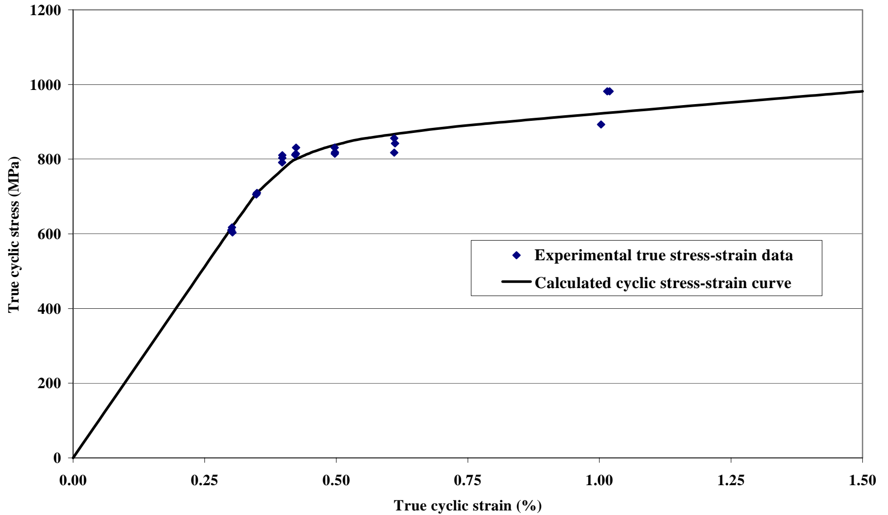
Figure 5. Cyclic stress-strain curve for 4140 Quenched and Tempered steel (Iteration 67).
