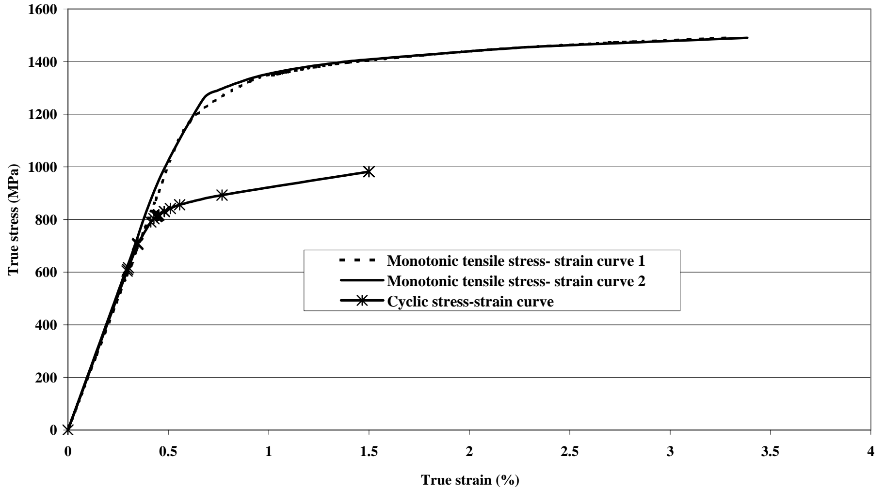
Figure 6. Monotonic and Cyclic stress-strain curves for 4140 Quenched and Tempered steel (Iteration 67).
