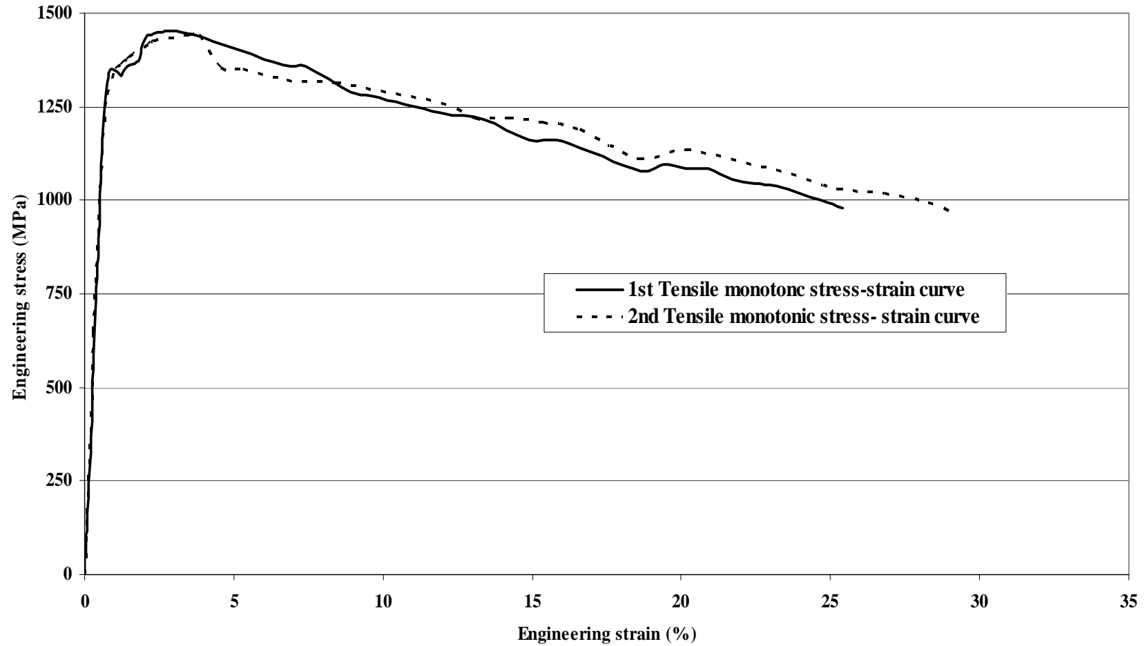
Figure 7. Tensile monotonic stress-strain curves for two 4140 Quenched and Tempered steel specimens (Iteration 67).
