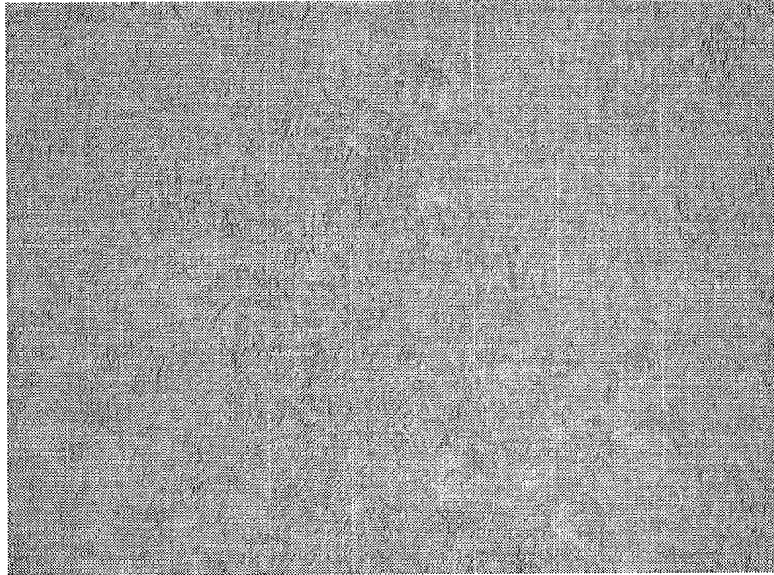
Figure 2: Photomicrograph in first longitudinal direction (L-T) at 500X for SAE 4620 Carburized Case steel (rolling direction is horizontal)
