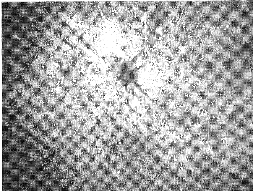
Figure 3c: Subsurface crack at 100X (zoom in) for SAE 4620 Carburized Case steel
