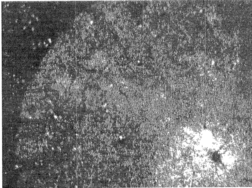
Figure 3b: Subsurface crack at 50X for SAE 4620 Carburized Case steel
