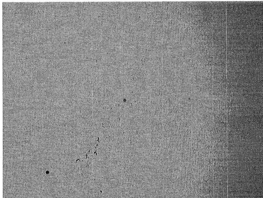
Figure 3a: Examples of inclusions in the first longitudinal direction (L-T) at 100X for SAE 4620 Carburized Case steel (rolling direction is horizontal)
