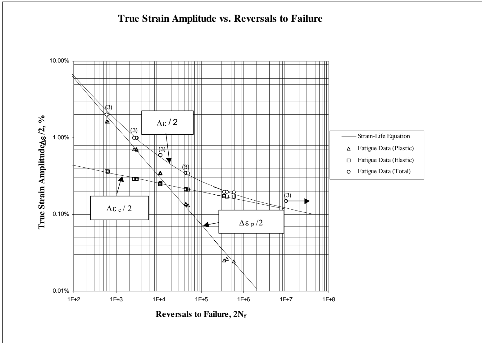
Figure 11: True strain amplitude versus reversals to failure
