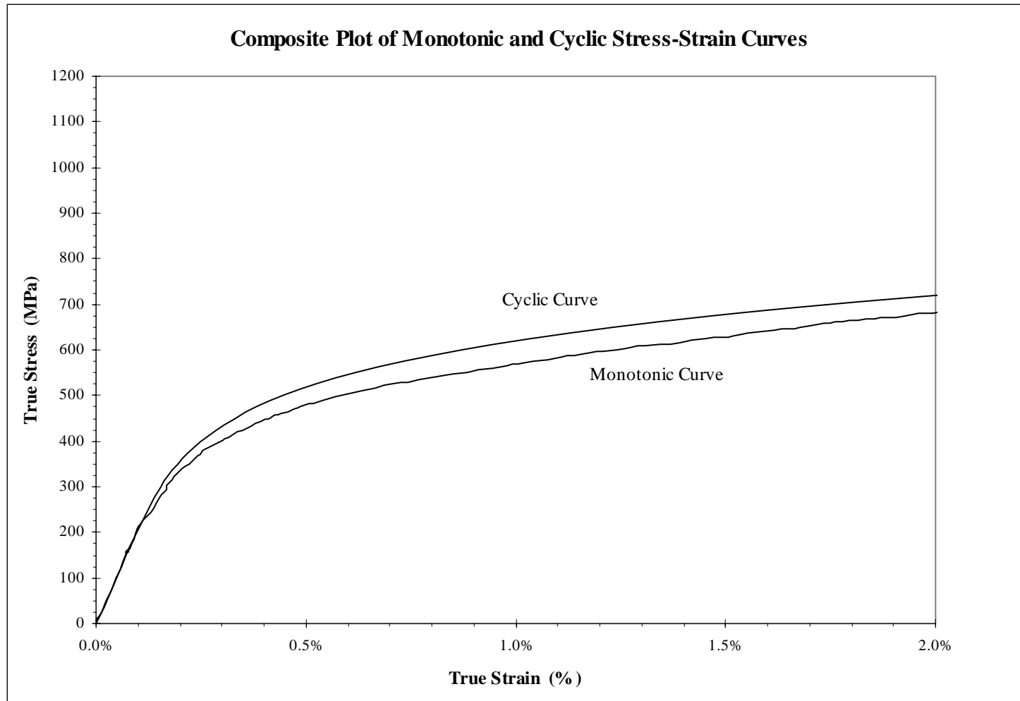
Figure 8: Composite plot of cyclic and monotonic stress-strain curves
