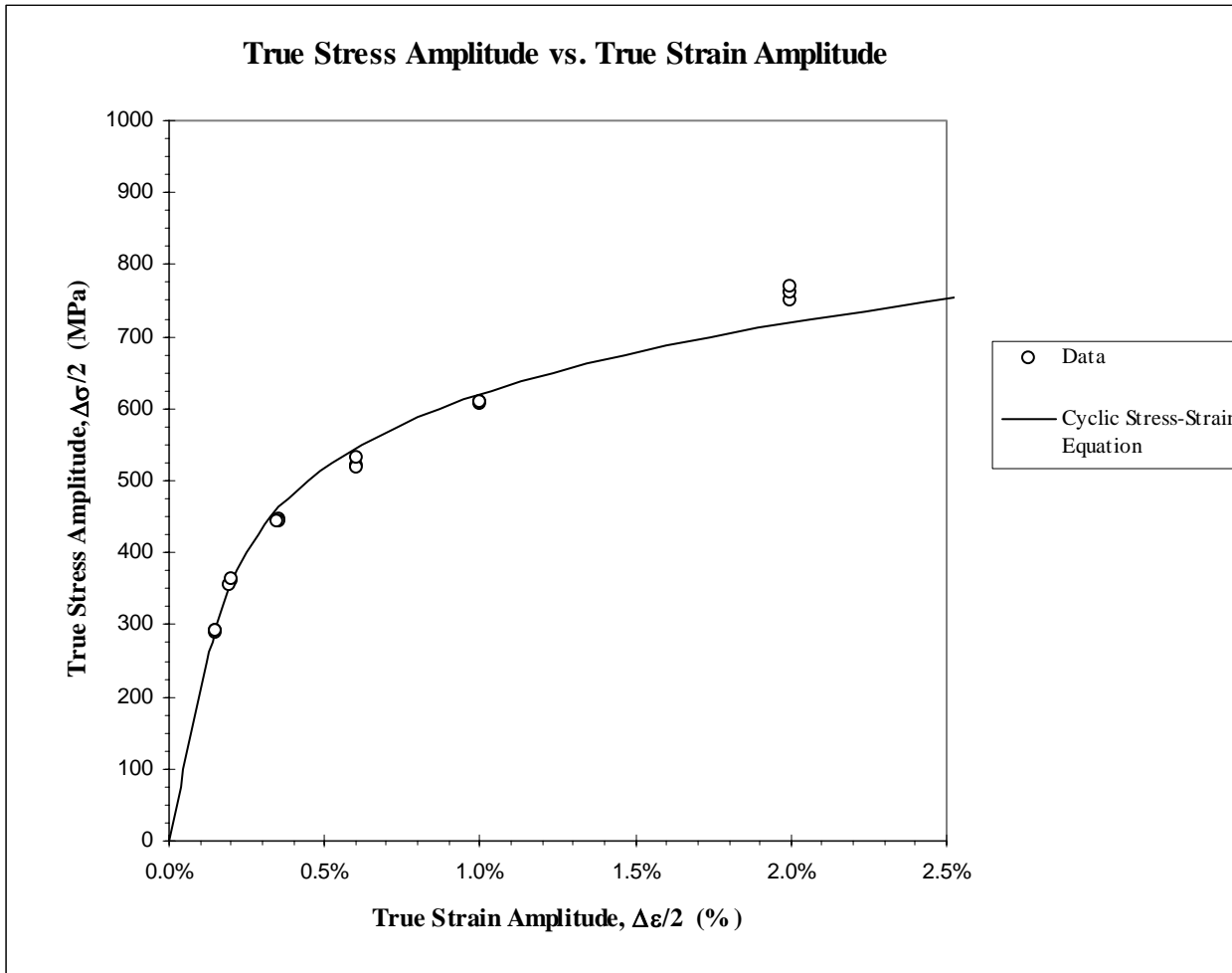
Figure 7: True stress amplitude versus true strain amplitude
