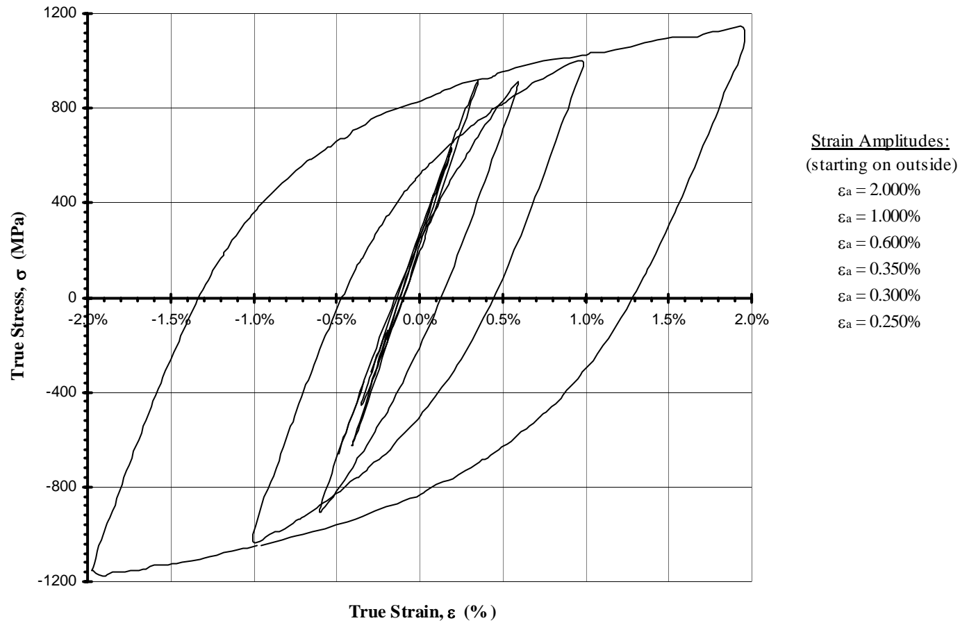
Figure A.2: Composite plot of midlife hysteresis loops
