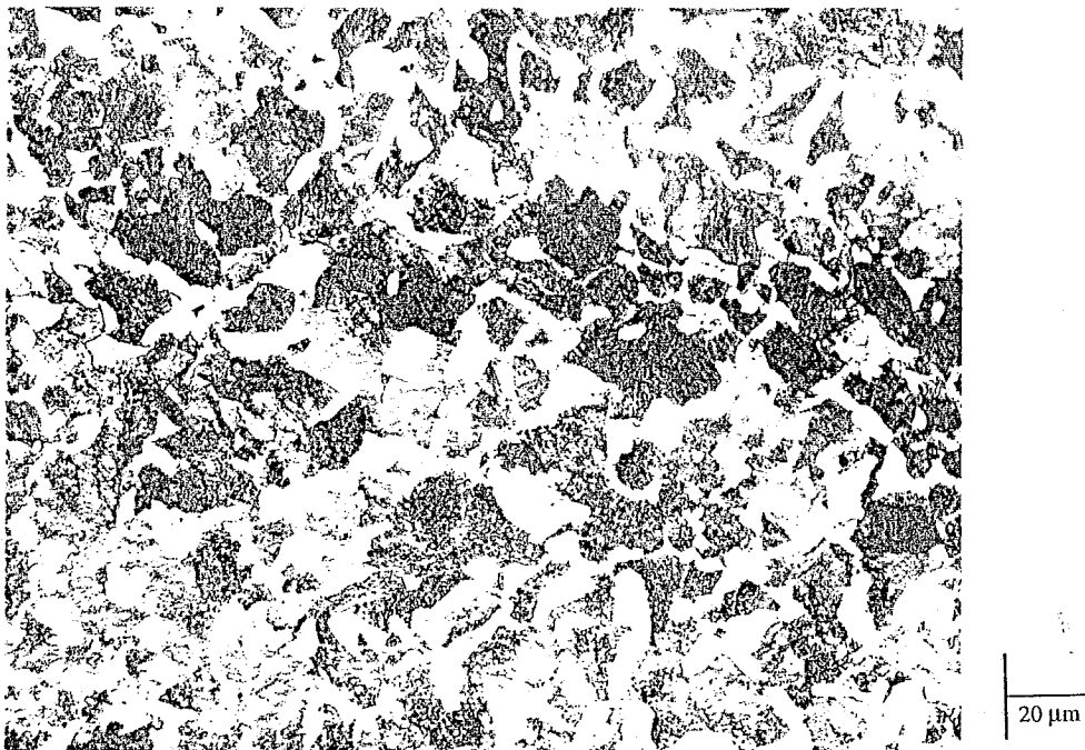
Figure 2b: Photomicrograph in the longitudinal direction (L-T) at 500X for SAE 10V45 normalized steel (rolling direction is horizontal)
