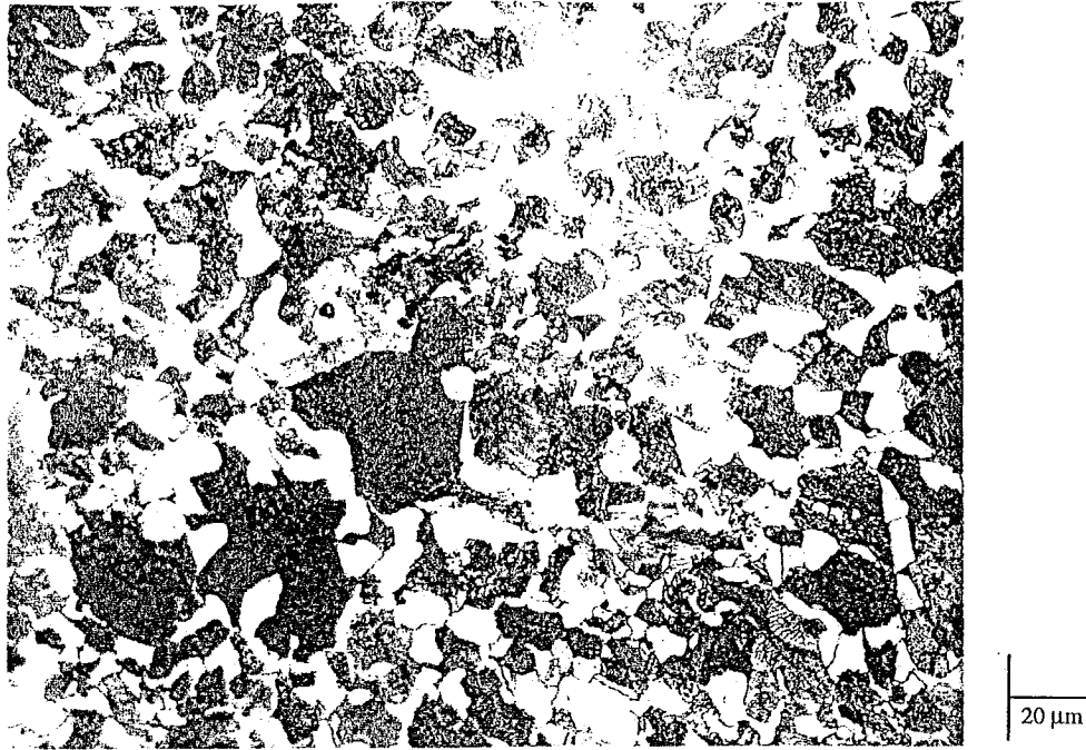
Figure 2a: Photomicrograph in the transverse direction (T-T) at 500X for SAE 10V45 normalized steel
