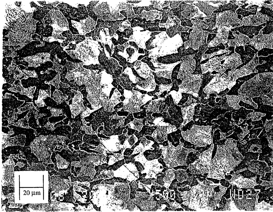
Figure 2: Photomicrograph in the longitudinal direction (L-T) at 500X for SAE 1038 cold size/form steel (rolling direction is horizontal)
