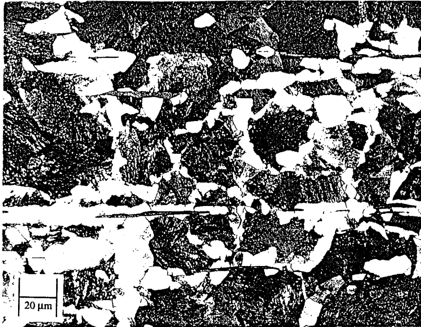
Figure 2: Photomicrograph in the longitudinal direction (L-T) at 500X for SAE 1141 (VFG) normalized steel (rolling direction is horizontal)
