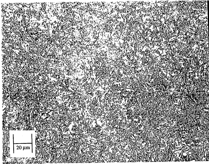
Figure 2: Photomicrograph in the longitudinal direction (L-T) at 500X for SAE 1141 (AIFG) Q&T steel (rolling direction is horizontal)
