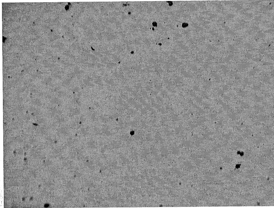
Figure 3: Examples of inclusions in the transverse direction (T-T') at 100X for SAE 10B21 Q&T Steel
