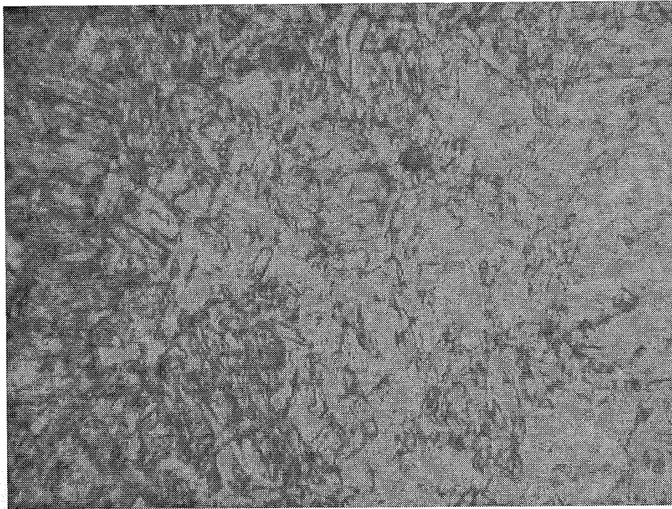
Figure 2: Photomicrograph in transverse direction (T-T') at 1000X for SAE 10B21 Q&T Steel
