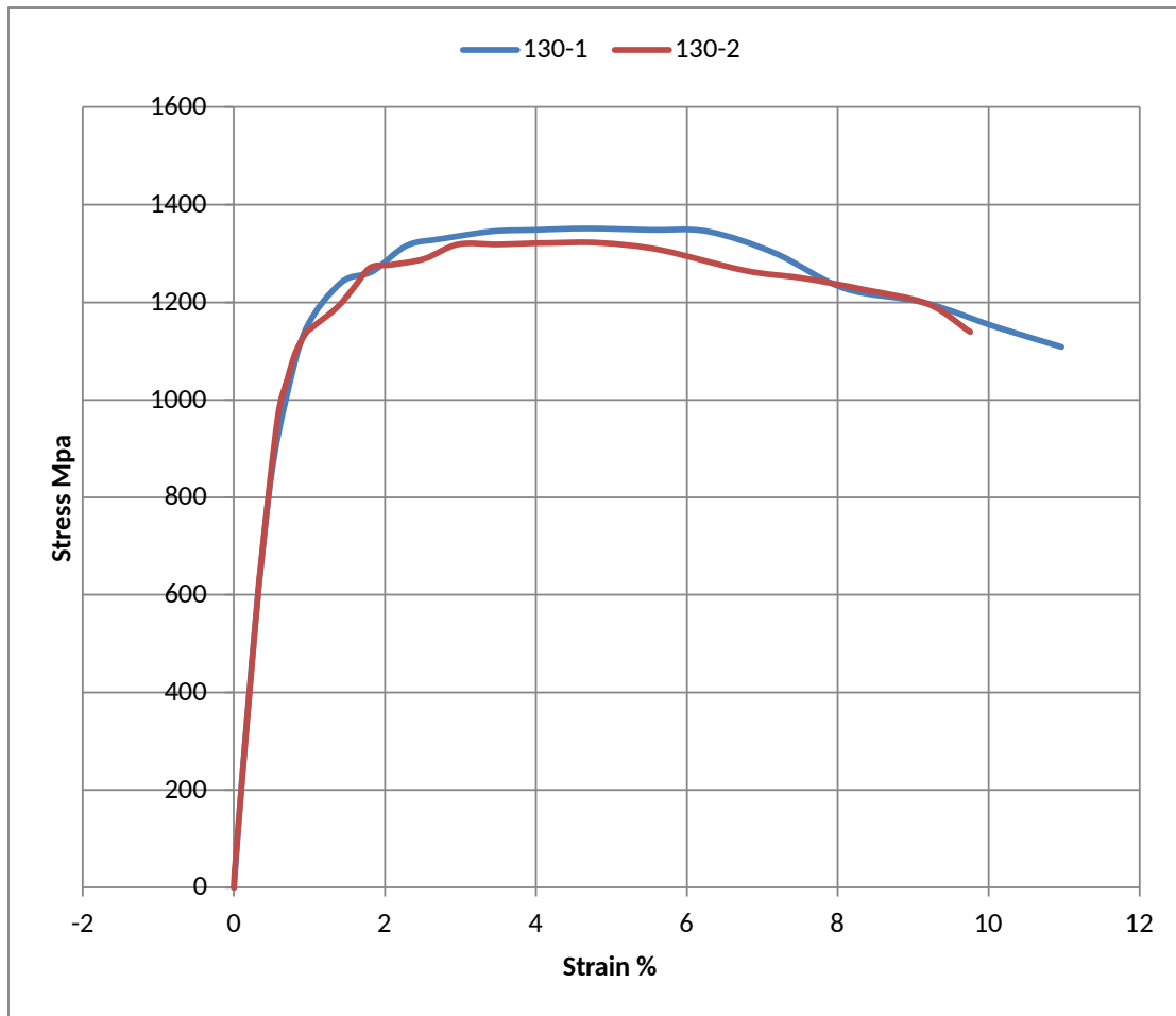
Figure 2: Monotonic engineering stress-strain curves for AISI 20MnCr5 (IT 130)
