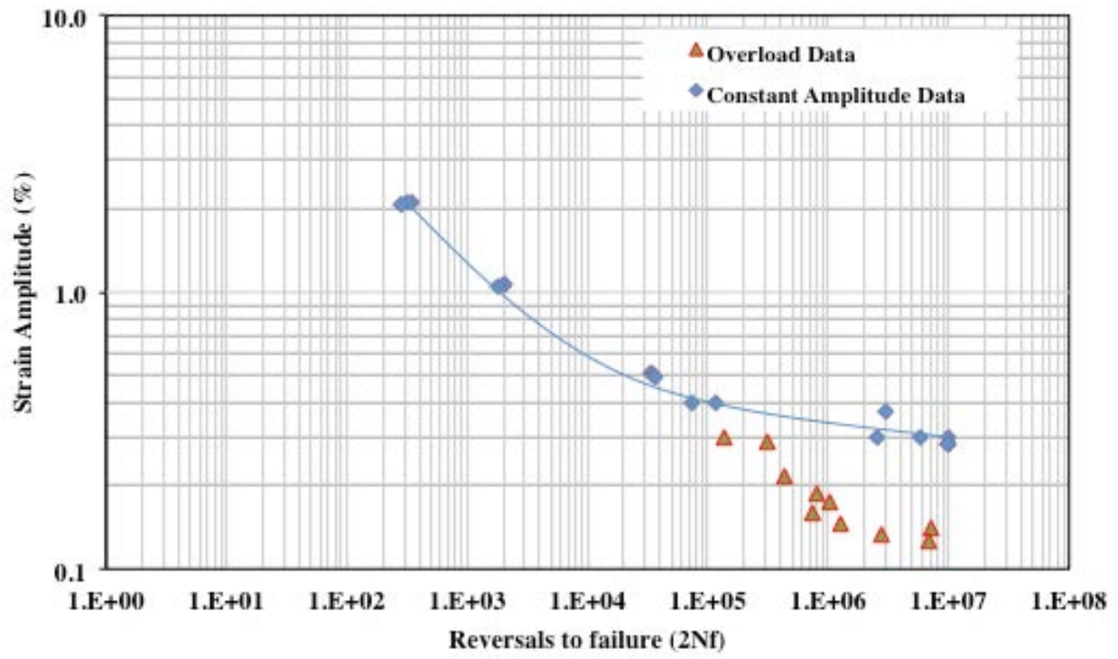
Figure 6: Overload and constant fatigue curves for AISI 20MnCr5 (IT 130)
